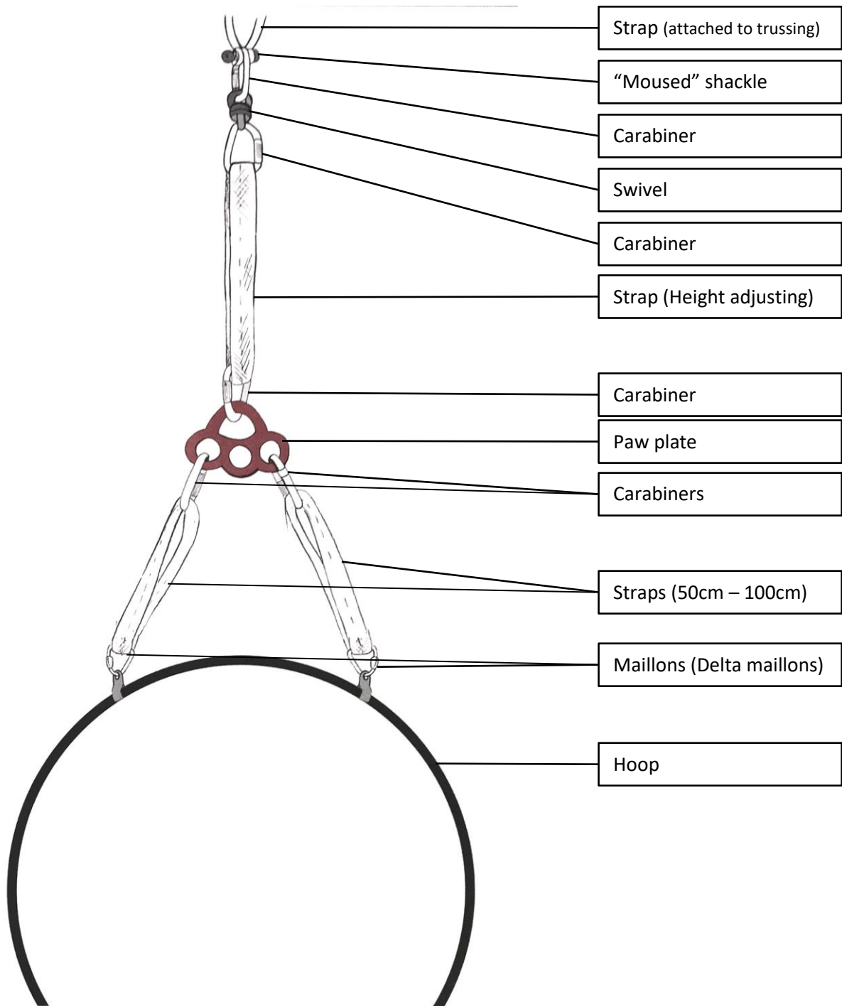
Rigging system
